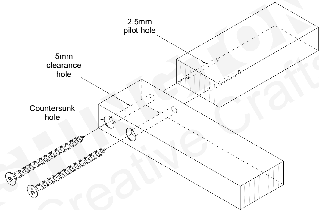
Exploded Joint
